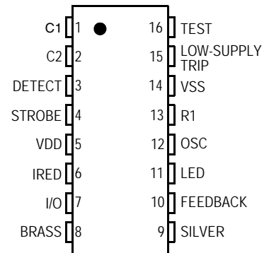
Figure 1. Pin Connections
